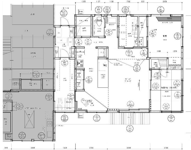
1floor plan
